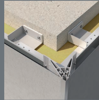
Attachment scenario: 90° corner
